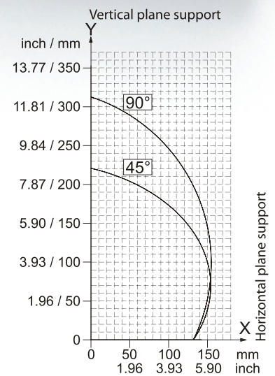
DTI 450 cutting diagram
